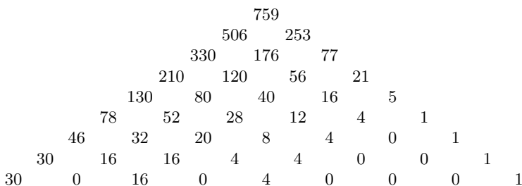
Fig. 5.1. The Leech triangle
